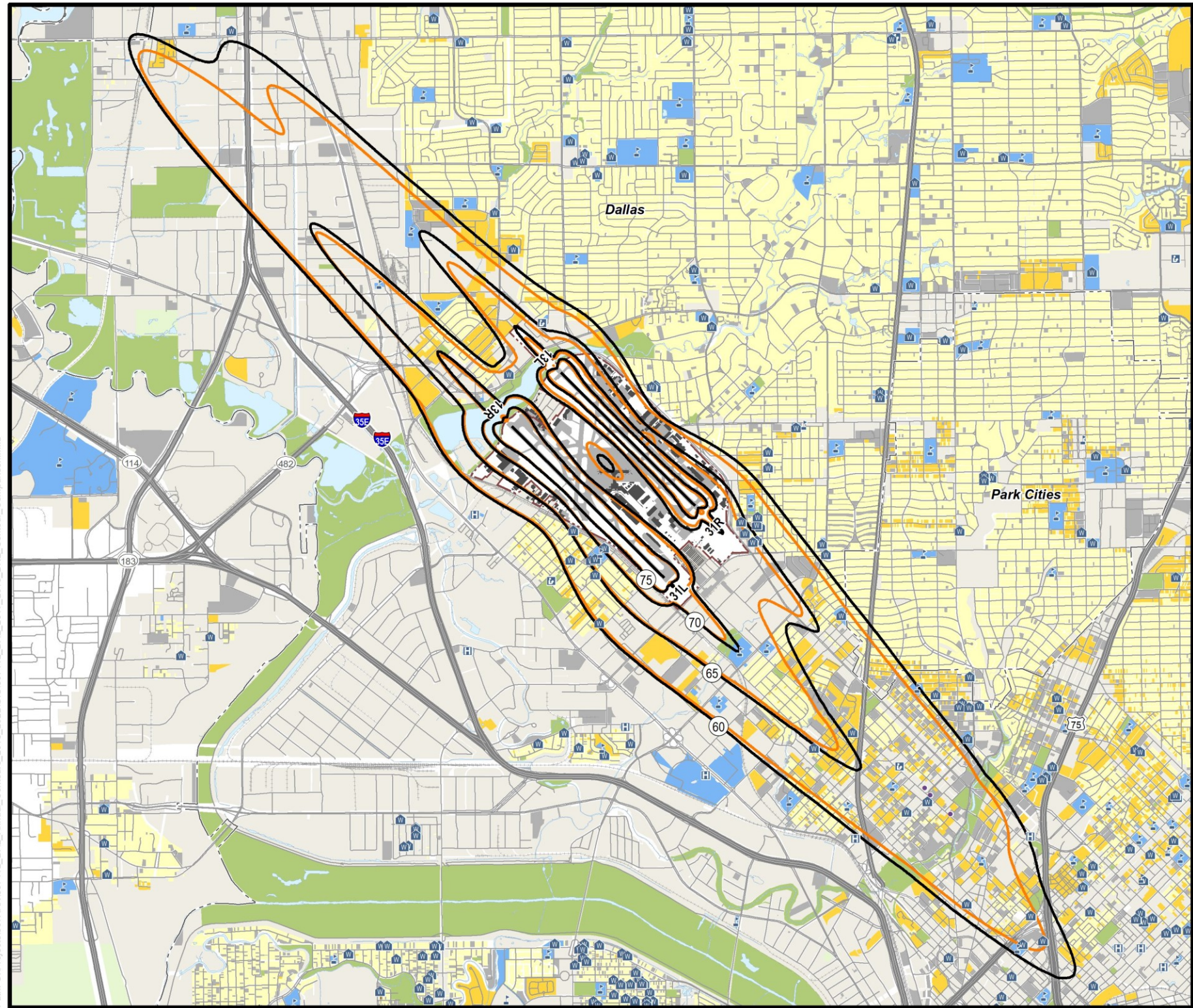
Figure 28. 2018 DNL Contours compared to 2017 DNL Contours
